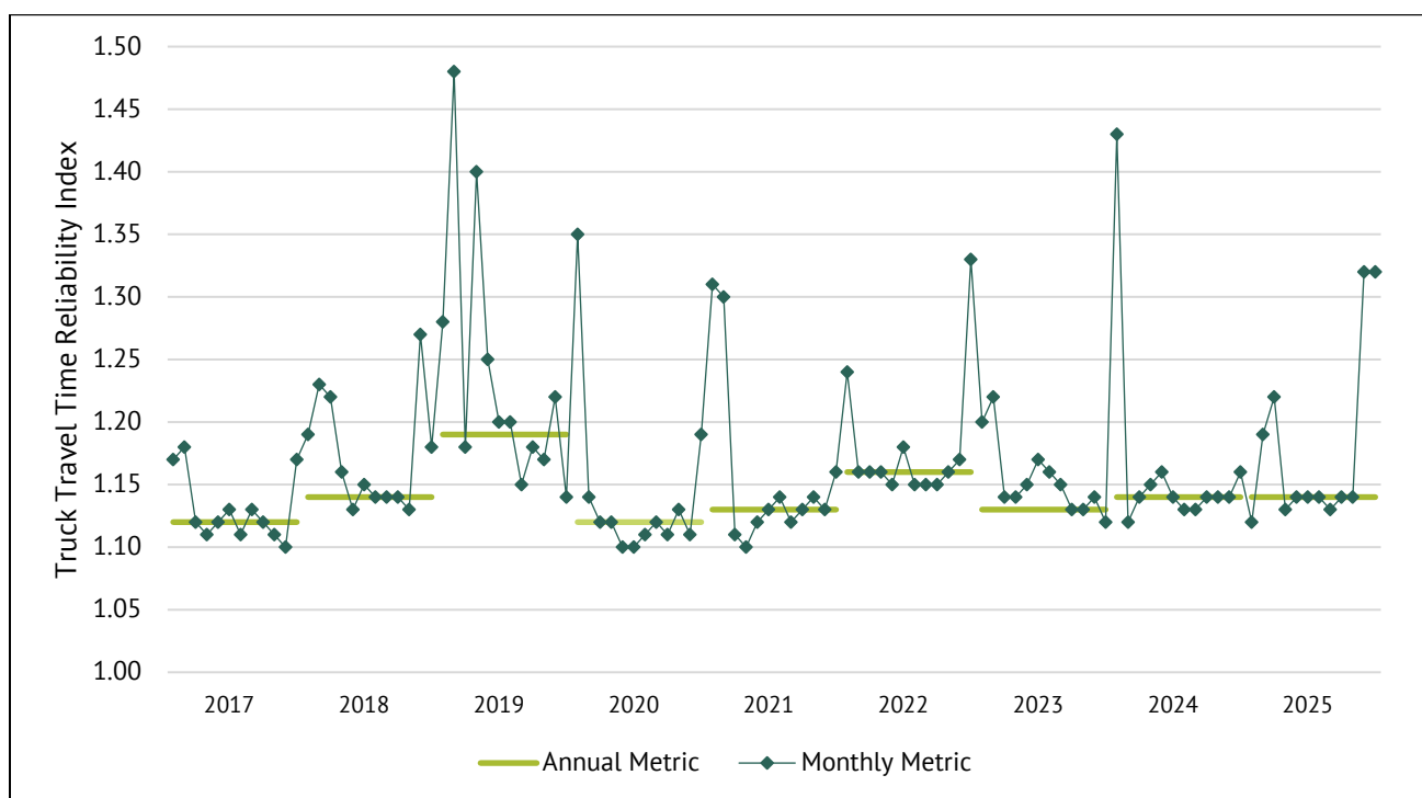
Figure 2: Historical annual and monthly Interstate Truck Travel Time Reliability (TTTR) Index (lower TTTR = higher reliability)
